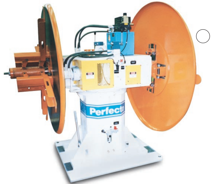
Model RD046012 with hydraulic expansion and hydraulic jog.
